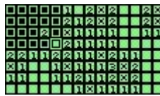
Minesweeper plugin
