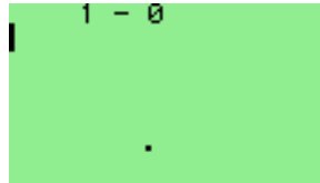
Pong game
