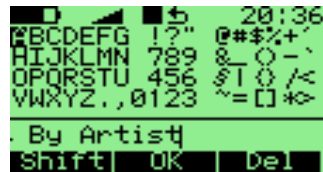
Recorder keyboard
