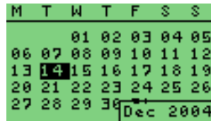
Calendar
