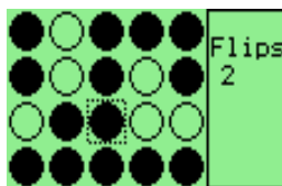
Flipit plugin
